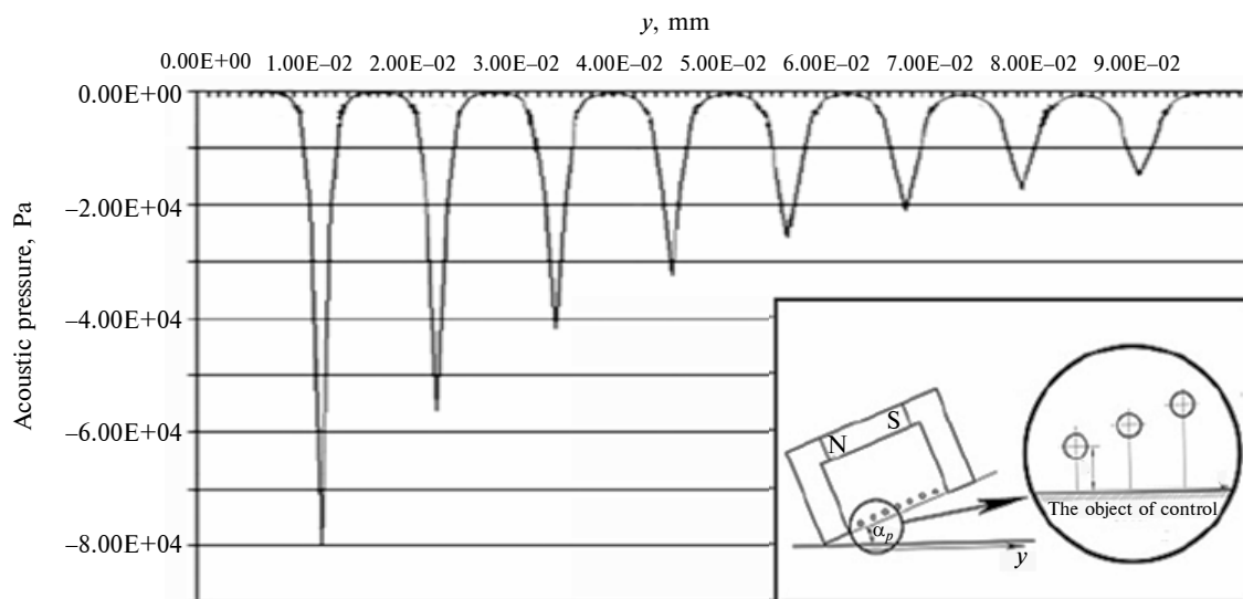
Fig. 9. Dependence of p_{\Sigma}(y) in the case of a distortion of the sensor by \alpha_p = 0,5^{\circ} in reference to the controlled object surface, B_{\perp} = 0,3 T, h = 1 mm, f_i = 0,5 MHz, I_0 = 2 A
