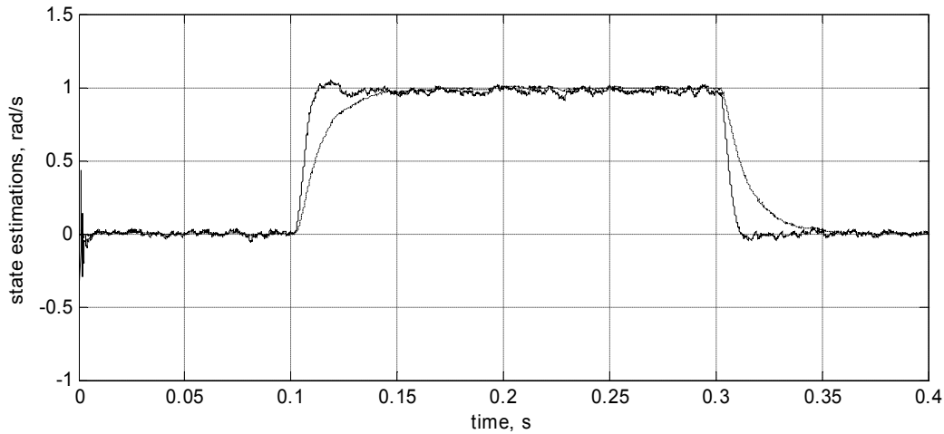
Fig. 4. State estimations over time (solid – input angular rate, dashed – output angular rate)
