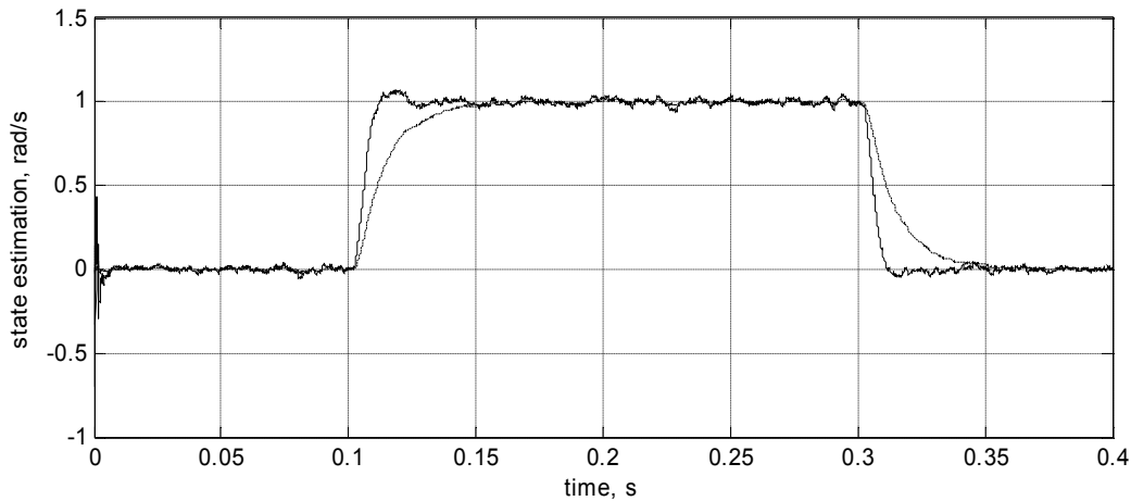
Fig. 3. State estimations over time (solid – input angular rate, dashed – output angular rate)
