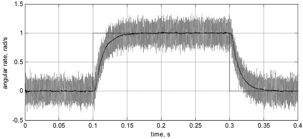
Fig. 2. Angular rate measurements (gray – noised output, dotted – actual output without noise, solid – output estimation)
