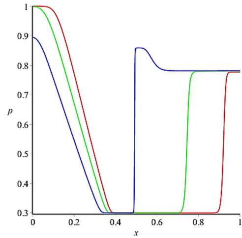
Fig. 5. The results of pressure calculations for the whole pipe at number of space element J = 500 ;
