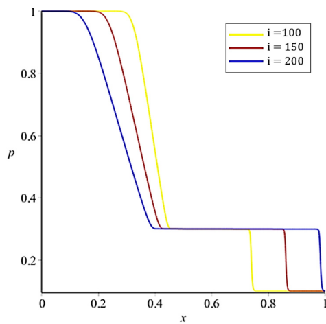
Fig 4. The results of pressure calculation for the same number of elements, time step interval, but for different time: a) for ii=100 , t = T_0 ; b) for ii=150 , t = 1.5T_0 ; c) for ii=200 , t = 2T_0
