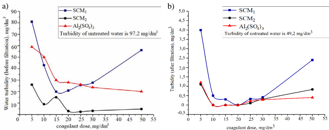
Fig. 1 Turbidity removal before (a) and after (b) filtration by SCM 1 , SCM 2 and Al 2 (SO 4 ) 3 coagulants accordingly
