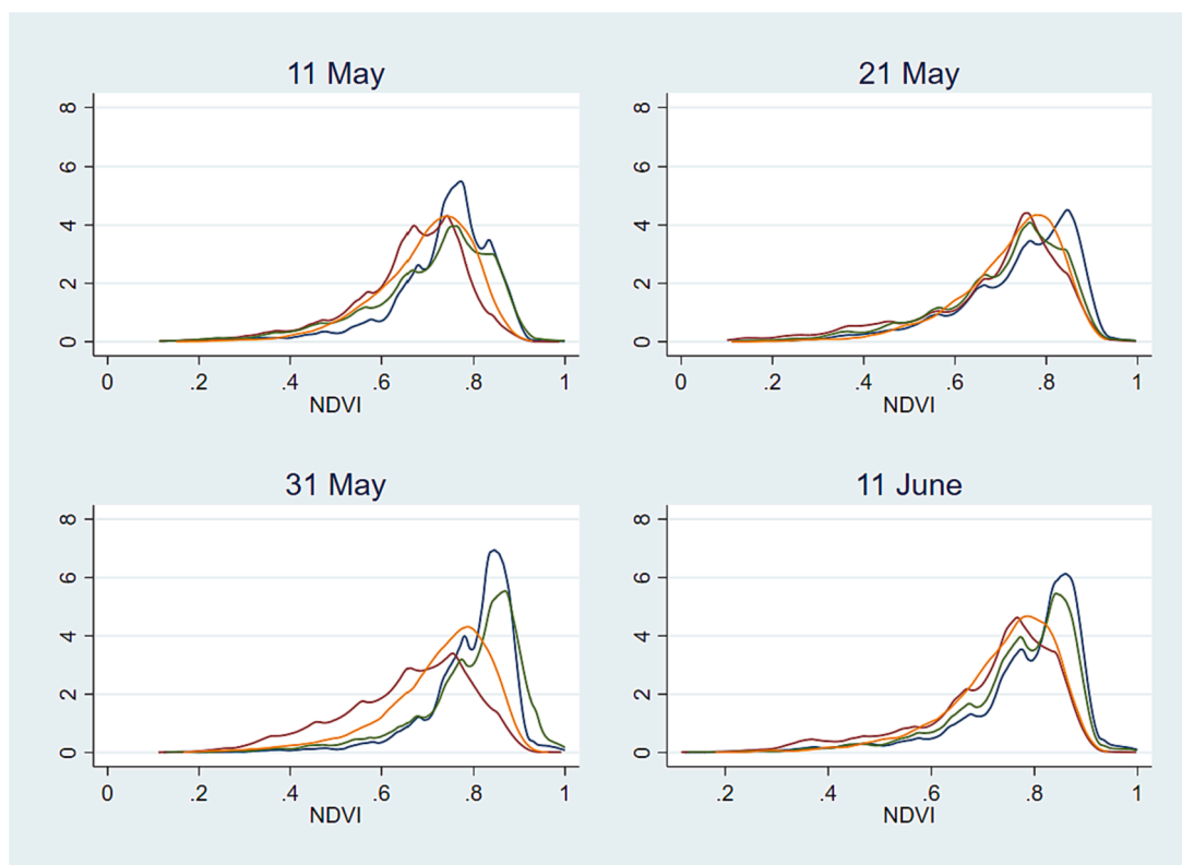
Fig. 3b. NDVI for fields grown with winter cereals at different dates during the growing season, 2019–22. Note: Blue = 2019; Red = 2020; Green = 2021; Orange = 2022. (For interpretation of the references to colour in this figure legend, the reader is referred to the web version of this article.)
