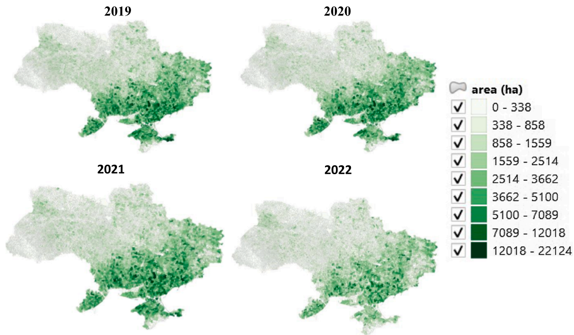
Fig. 2. Map of winter crop cover for 2019 to 2022 growing seasons.
