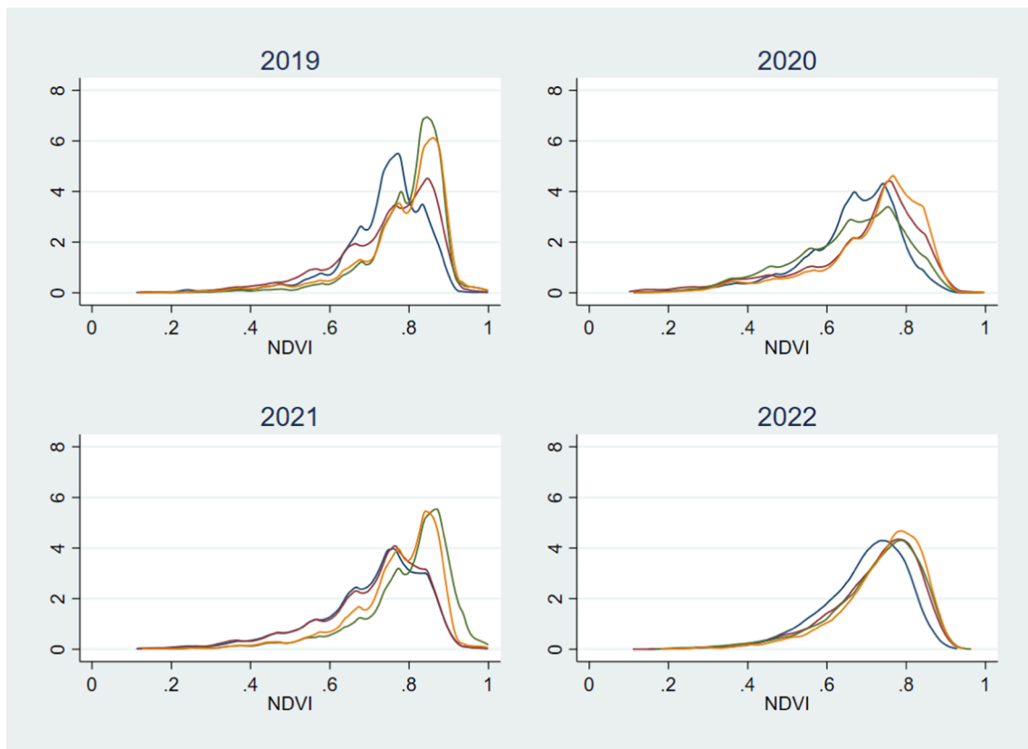
Fig. 3a. Density of NDVI for fields grown with winter cereals for different time periods, 2019–22. Note: Blue = May 1–11; Red = May 12– 21; Green = May 22–31 Orange = June 1–11. (For interpretation of the references to colour in this figure legend, the reader is referred to the web version of this article.)
