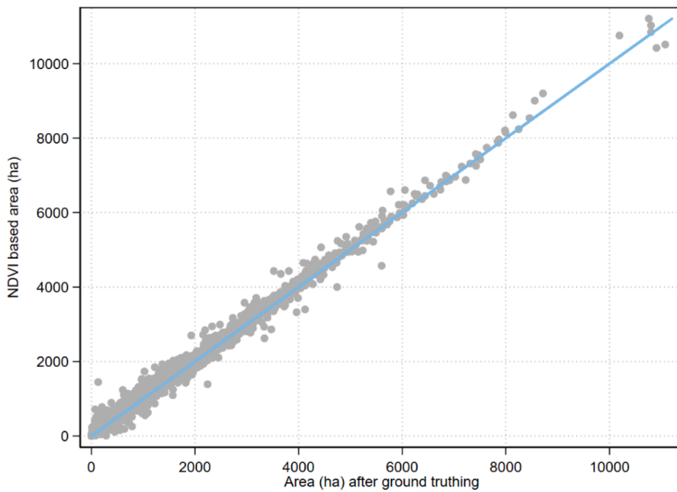
Fig. A4a. Comparison of village-level winter crop area based on NDVI segmentation on May 1 vs ground truthed data, 2022.
