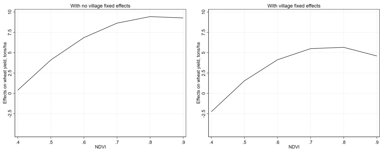
Fig. A5. Predicted marginal effects of peak NDVI on wheat yield for Ukraine Source: Computed based on coefficients estimated in Appendix Table A9.
