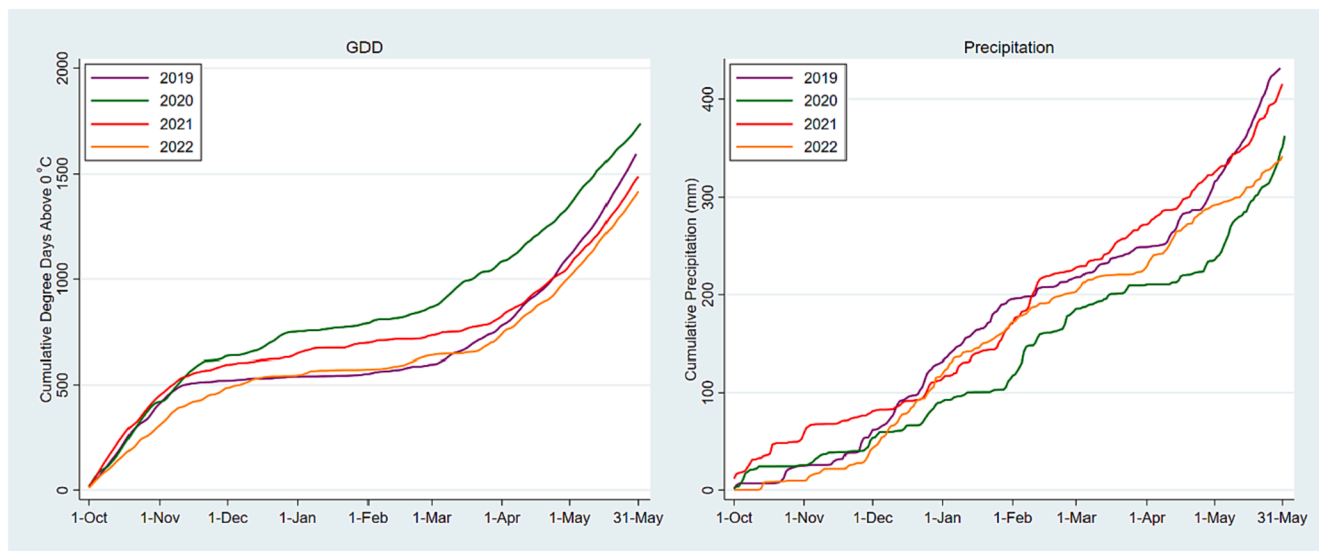
Fig. 4. Cumulative mean growing degree days (GDD) above 0 °C and daily rainfall October 1 – May 31.
