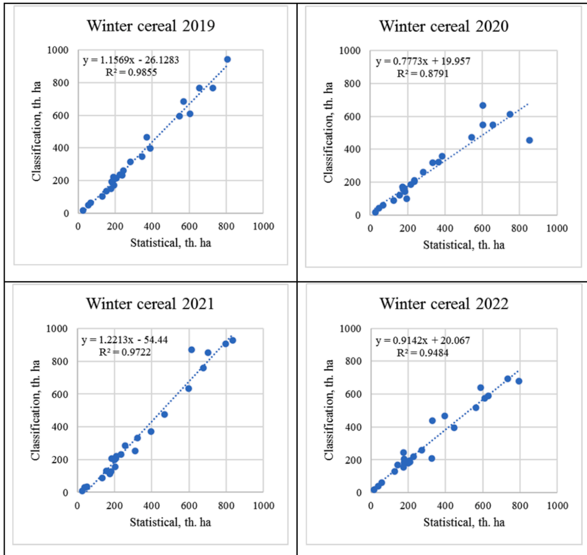
Fig. A3. Comparison of winter cereal area based on interpretation of remote sensing to official statistics at oblast level.
