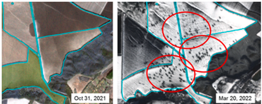
Fig. A2. Examples of most frequent types of field damages.
