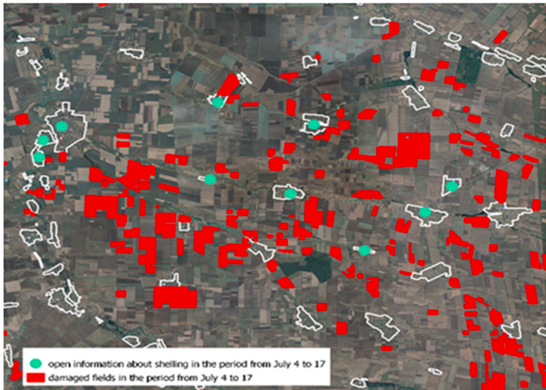
Fig. A1. Comparing location of damaged fields determined based on Satellite imagery to locations of military action based on ACLED data.
