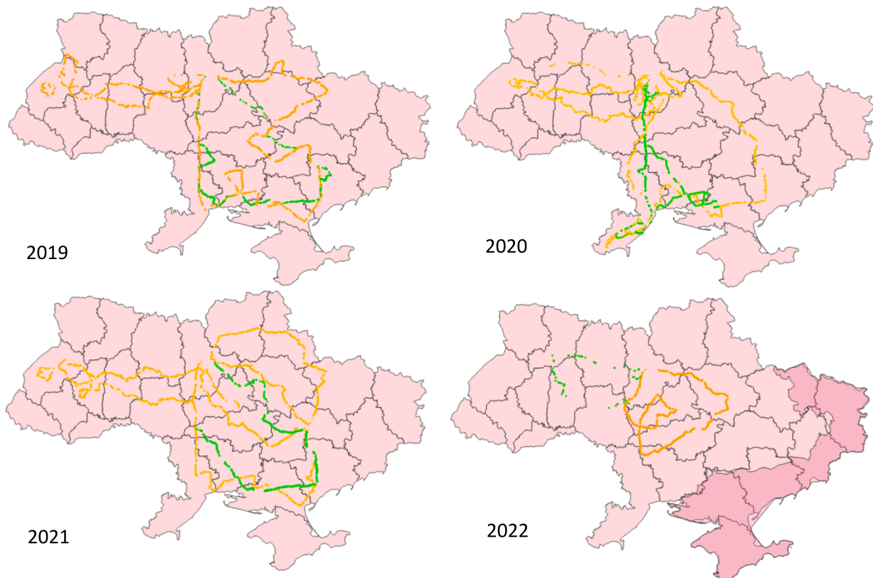
Fig. 1. Routes for in-situ training data collection, 2019–2022. Note: Green and orange refer to the paths of ground data collection for winter and summer crops, respectively. Area in a darker shade of red is currently occupied by Russian forces. (For interpretation of the references to colour in this figure legend, the reader is referred to the web version of this article.)
