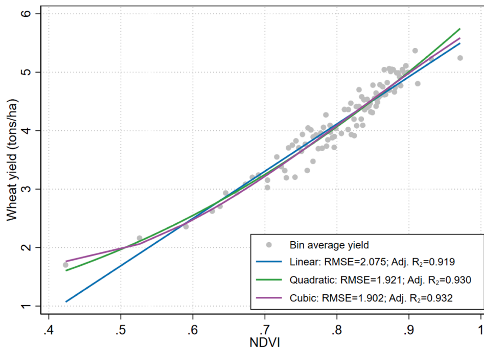
Fig. A4b. Relationship between winter wheat yield and peak NDVI: 2019–2020 Note: For each of the two years, we classify yield in 50 equally spaced bins and link these to the associated NDVI.
