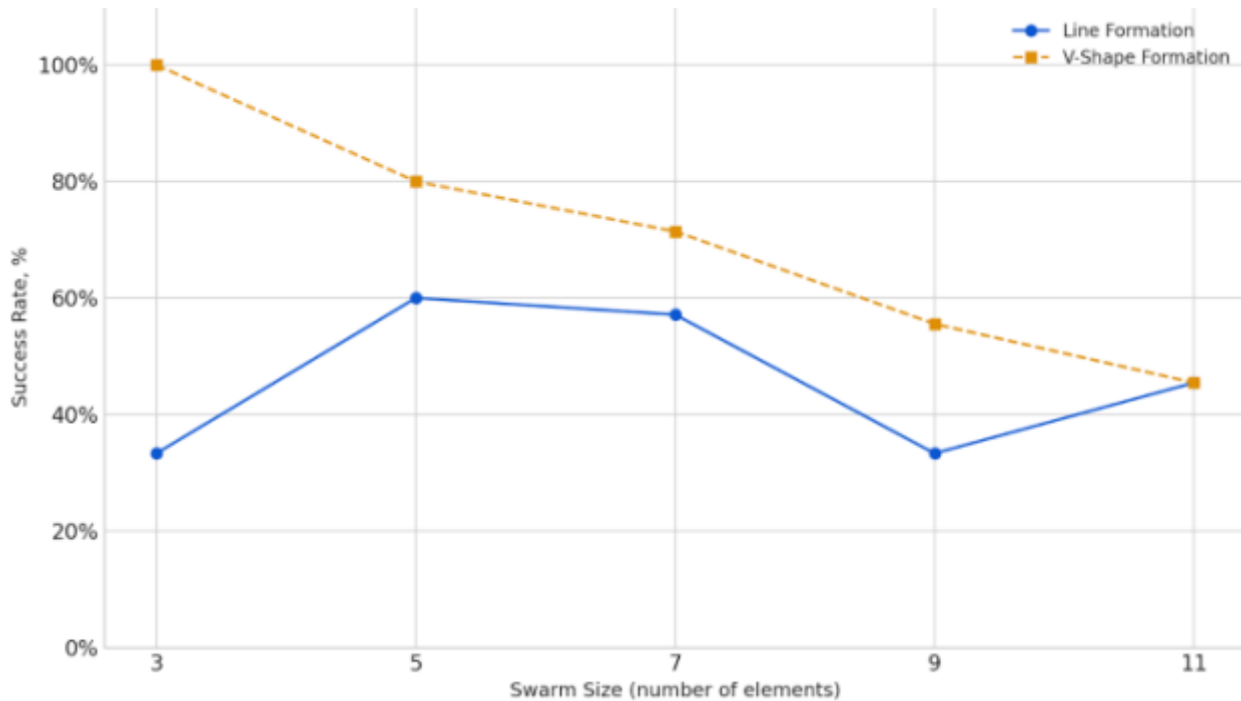
Fig. 5. Success rate of the hybrid algorithm depending on the formation size and type.
