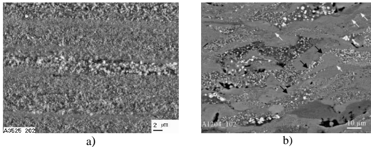
Fig. 4 – SEM images of cross-sectional microstructure for (a) extruded rod (b) cold-sprayed alloy, both performed by Al_{94}Fe_3Cr_3 -feedstock powder. Black arrows in (b) indicate the evidence of shear instabilities at the particle/particle boundaries whereas white arrows indicate the local metallurgical bonding between the powder particles due to impact fusion.
