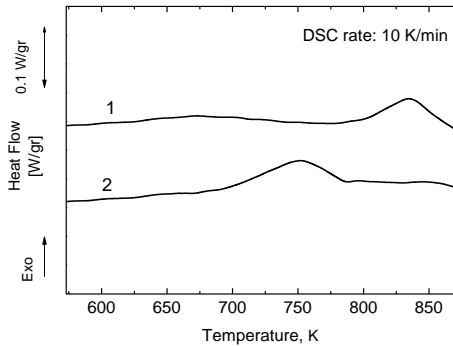
Fig. 3 – DSC traces recorded at the heating rate 10 K/min for (1) Al 94 Fe 3 Cr 3 feedstock powder and (2) as-extruded Al 94 Fe 3 Cr 3 alloy
