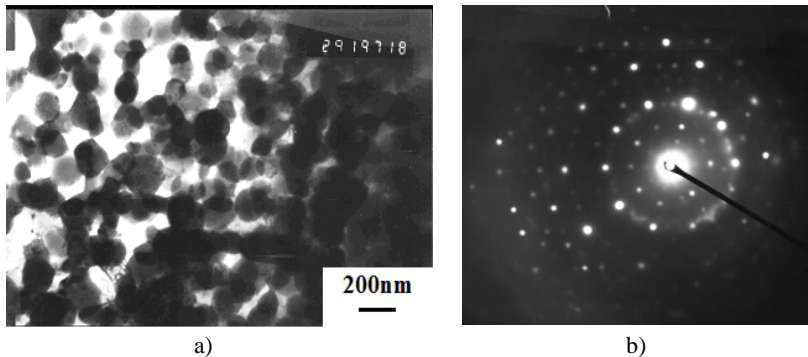
Fig.2 – (a) Bright field TEM image and (b) SAED pattern of the Al 94 Fe 3 Cr 3 alloy
