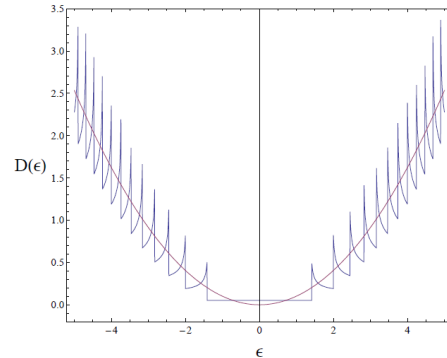
Fig. 2. Density of states
